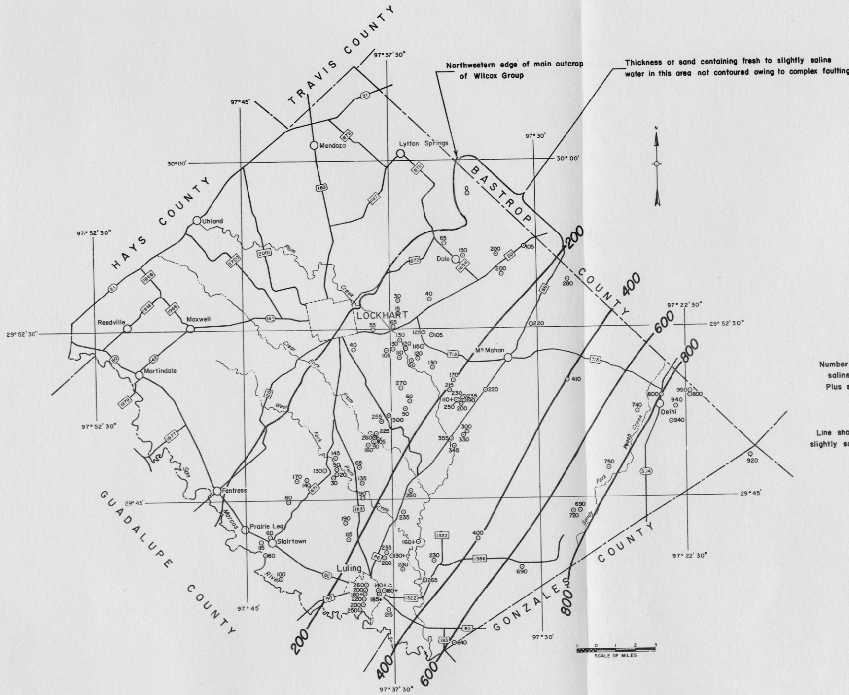
Figure 16 Approximate Thickness of Sand Containing Fresh to Slightly Saline Water in the Carrizo Sand and Wilcox Group
